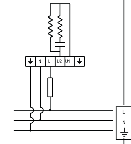
SCHEMA COLLEGAMENTO WIRING DIAGRAM
